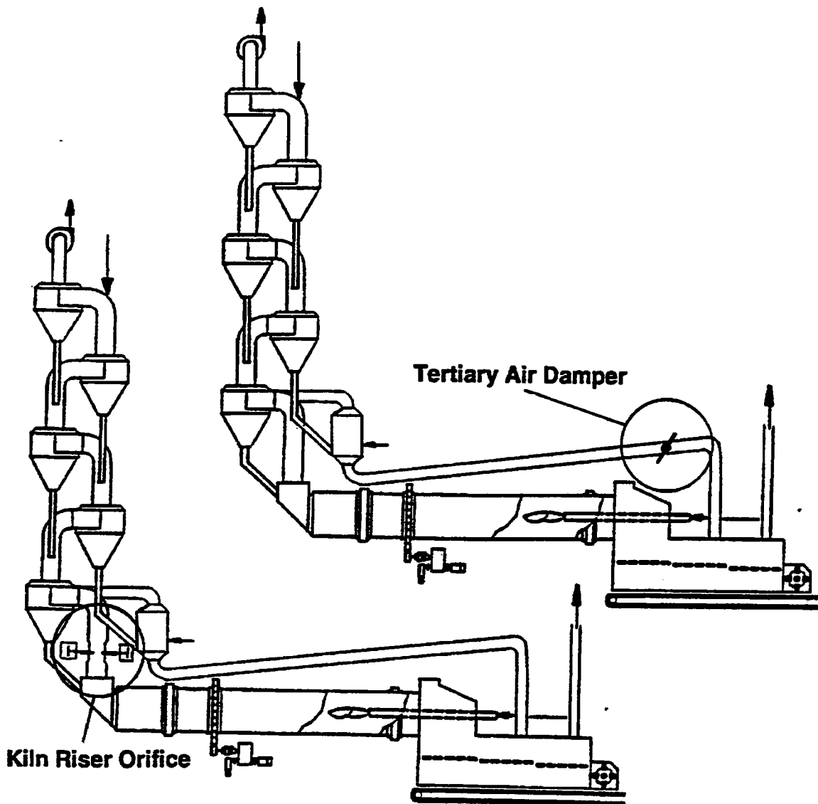
Fig. 10 TA Damper and Kiln Orifice
